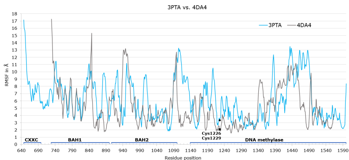
Figure 22. Comparison of residual movement within 4WXX, 3PTA, and 4DA4. RMSF chart for each protein structure was obtained in RStudio using Bio3D package (32). X-axis shows residue position and Y-axis stands for RMSF values in Å. Graphs were overlapped using Excel tools: A) RMSF comparison for 4WXX and 3PTA, B) RMSF comparison for 4WXX and 4DA4, C) RMSF comparison for 3PTA and 4DA4. Orange line is for 4WXX, blue line is for 3PTA and gray line is for 4DA4. Domains are named under the RMSF line. Active site cysteine (Cys1226, Cys1229) is marked with black dot on each line.
