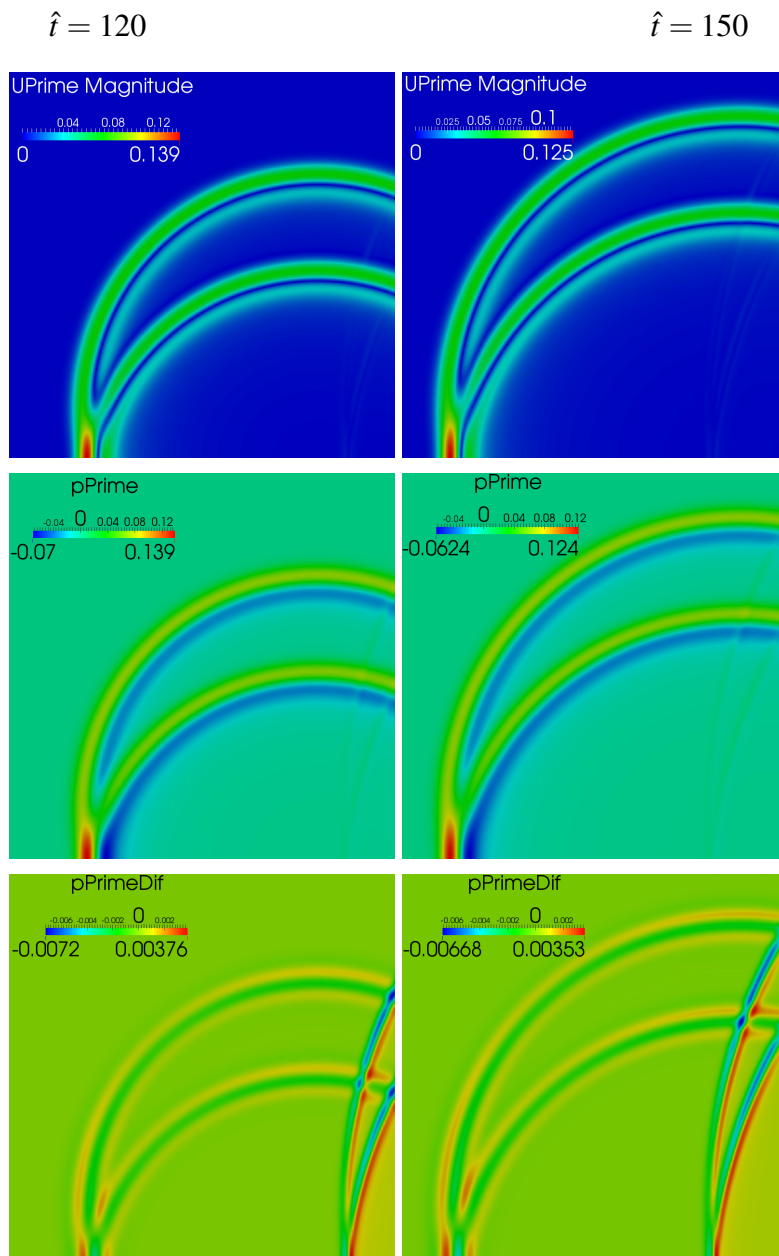
Figure 6.1.15: Acoustic fields: velocity fluctuation magnitude, |\hat{\mathbf{U}}' (top), pressure fluctuation, \hat{p}' (middle), difference between \hat{p}'_{analytical} and \hat{p}'_{numerical} (bottom), 1 000 000 cell grid.
