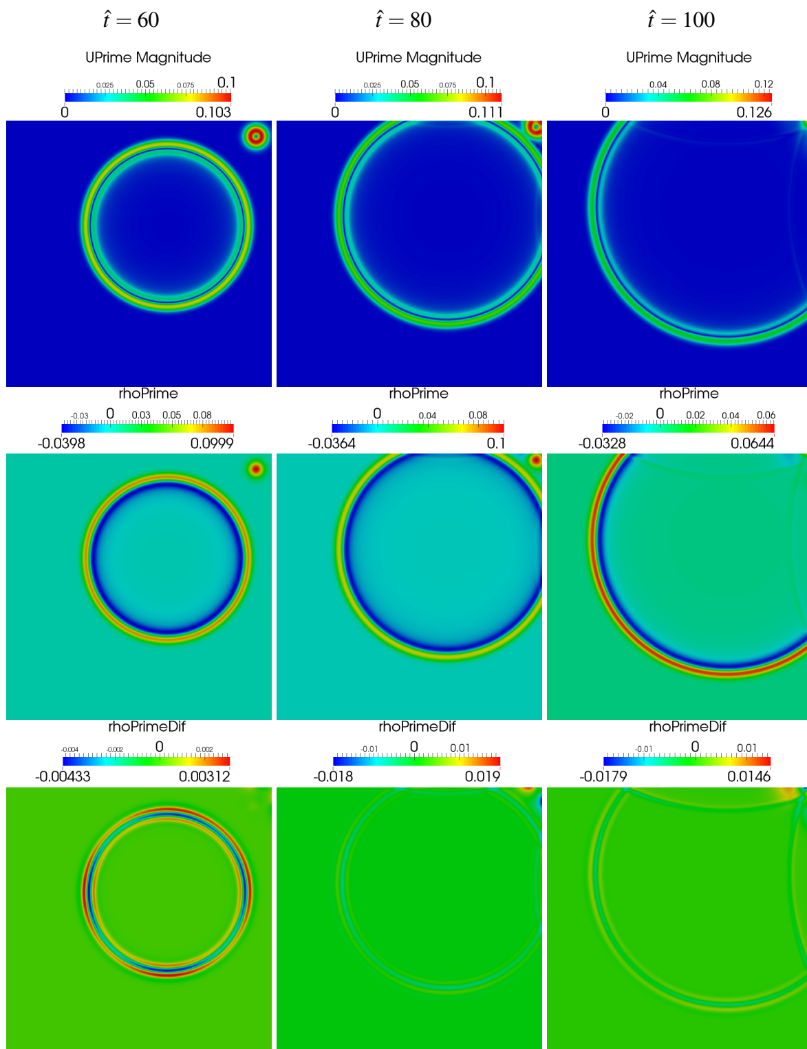
Figure 6.1.8: Acoustic fields: velocity fluctuation magnitude, |\hat{U}'| (top), density fluctuation, \hat{\rho}' (middle), difference between \hat{\rho}'_{analytical} and \hat{\rho}'_{numerical} (bottom), 1 000 000 cell grid.
