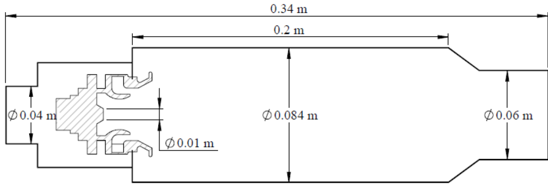
Figure 3.1: Combustor dimensions [43]
