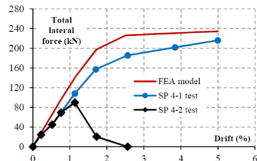
Figure 2.15: Lateral force–drift curve SP4 (Seco, 2019)
