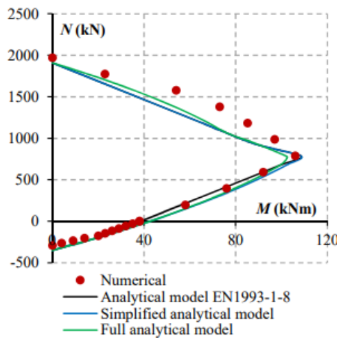
Figure 3.8: M - N interaction curves for P1 (Seco, 2019)
