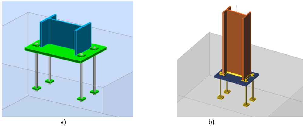
Figure 5.17: Software designs for PC4 test in a) Robot and b) IDEA StatiCa
