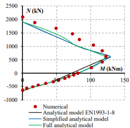
Figure 3.13: M - N interaction curves for P6 (Seco, 2019)
