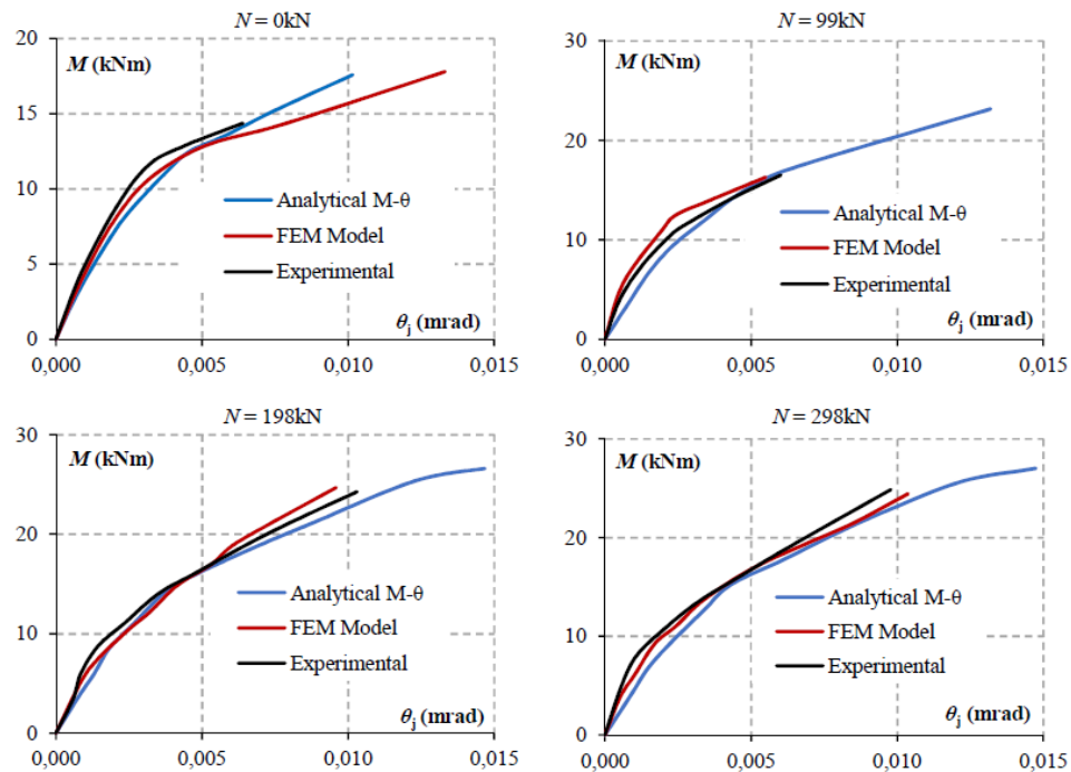
Figure 2.12: Experimental, numerical and analytical moment-rotation curves (SP1 tests) (Seco, 2019)
