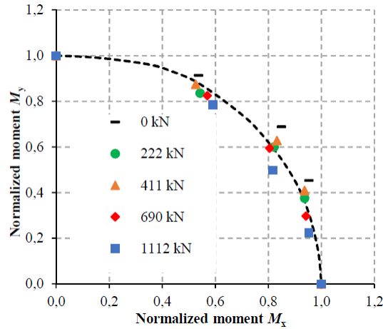
Figure 2.21: Proposed elliptical curve (Fasaei et al., 2018)
