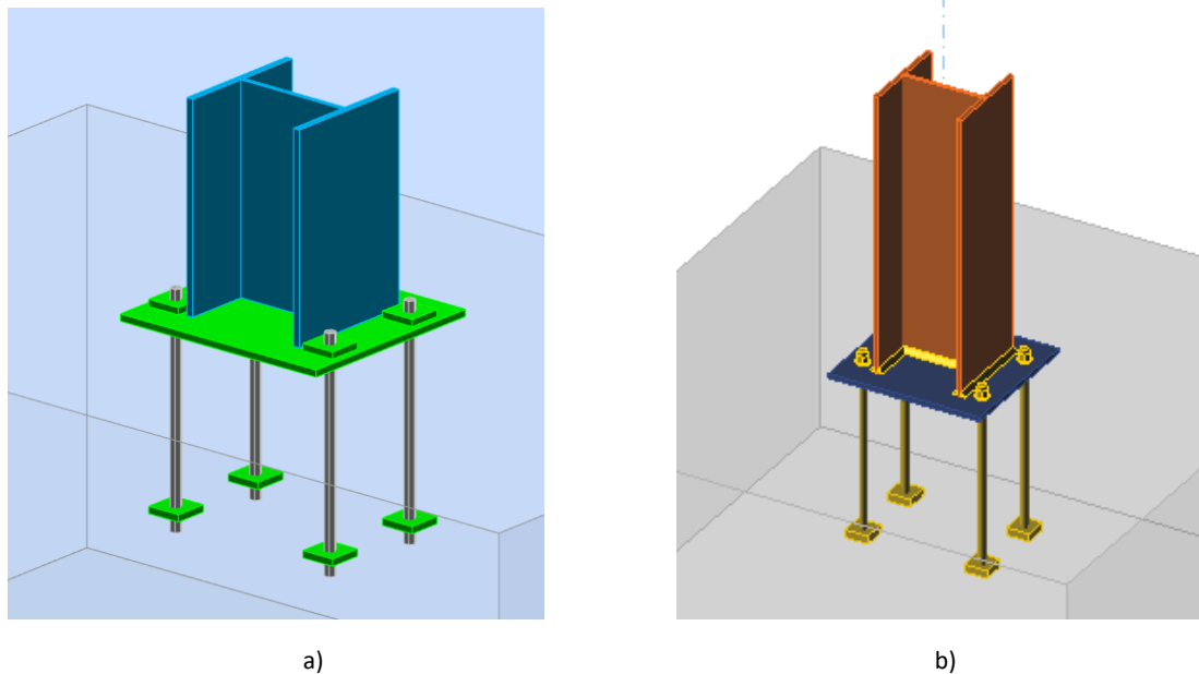
Figure 5.3: Software designs of the connection – a) Robot Structural Analysis , b) IDEA StatiCa
