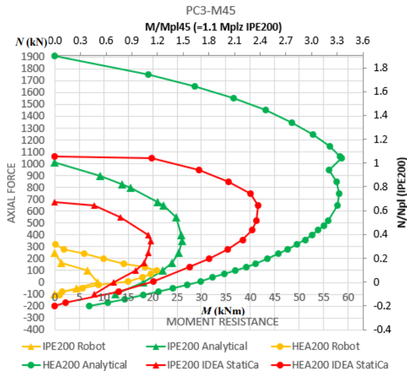
Figure 5.16: PC3-M45 moment resistance curves
