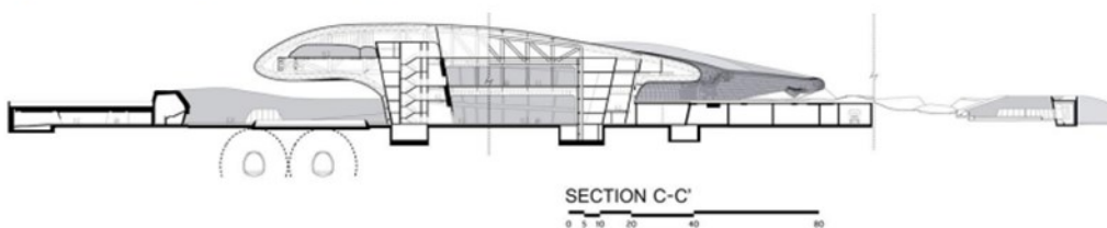
Figure 4.18: Dongdaemun Design Plaza section C-C'. 133
