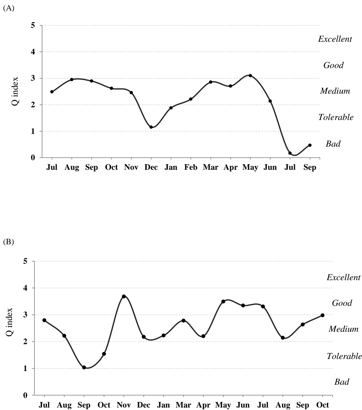
Figure 14. Dynamics of Q index and ecological status evaluation of Lake Sakadaš during the period of July 1972-September 1973 (A) and July 2011-October 2012 (B).
