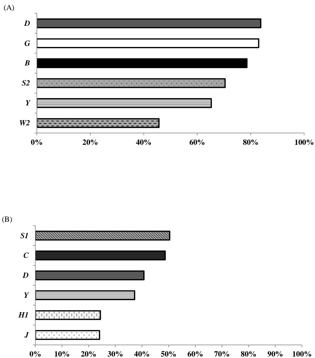
Figure 12. The maximal contribution to total biomass of best developed functional groups in Lake Sakadaš during the period of July 1972-September 1973 (A) and July 2011-October 2012 (B).
