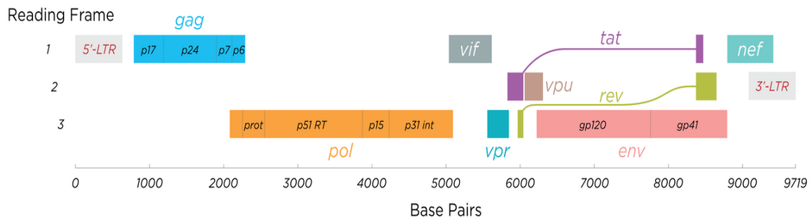
Figure 2: HIV-1 genome containing the structural genes (gag, pol, env), regulatory genes (tat and rev), and accessory regulatory genes (vpr, vif, nef, vpu). The work of Thomas Spletstoeser ( www.scistyle.com ).
