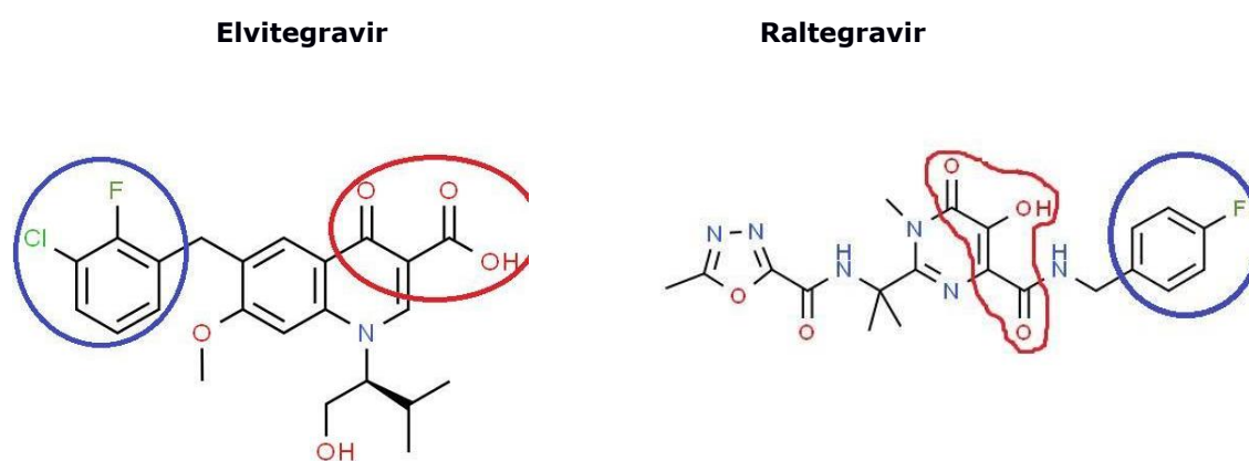
Figure 11: Structure and activity of Elvitegravir and Raltegravir. A halobenzyl group in a hydrophobic pocket (blue circle) and a triad that will chelate the two Mg 2+ ions (red circle) are visible. Taken and adapted from ChemSpider.
