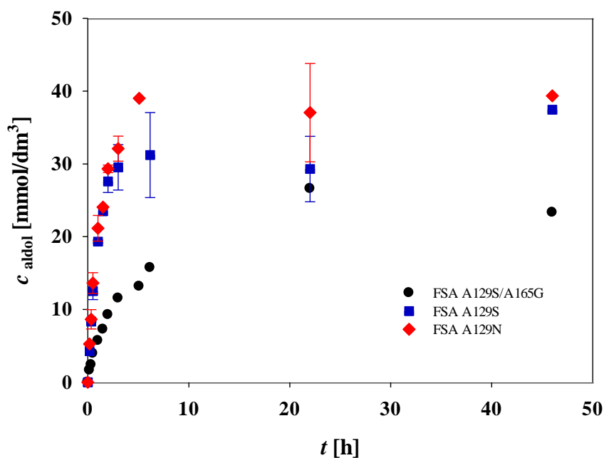
Slika 5.1. Aldolna adicija DHA na N-Cbz-glicinal u kotlastom reaktoru katalizirana s tri aldolaze ( \gamma_{\text{FSA}} = 0,5 \text{ mg/cm}^3 , c_{\text{N-Cbz-glicinal}} = 43 \text{ mmol/dm}^3 , c_{\text{DHA}} = 45 \text{ mmol/dm}^3 , 10 % (v/v) acetonitrila i 50 \text{ mmol/dm}^3 TEA-HCl pufer pH 8,0, 25^\circ\text{C} , V_{\text{reaktor}} = 0,5 \text{ cm}^3 ).
