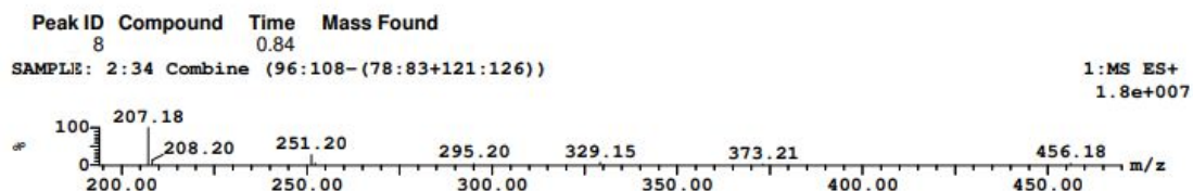
Fig. 12. MS spectra of desired product.
