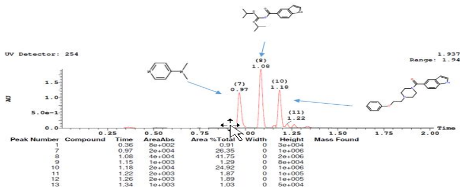
Fig. 17. UPLC-UV of reaction mixture of amidation.
