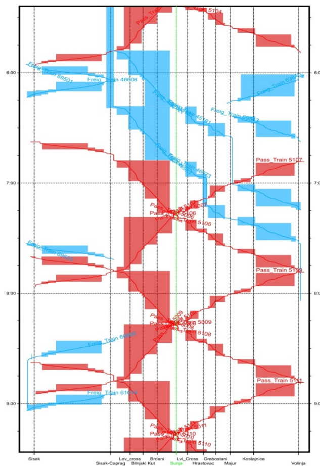
Figure 26. Clock-phase timetable
