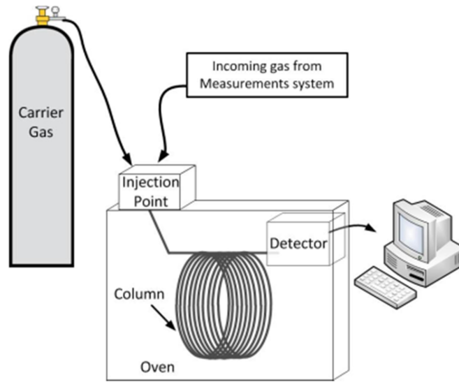
Figure 16- Gas chromatograph [36]
