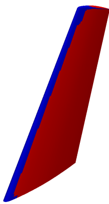
Figure 5.4.3: Body-fitted Onera M6 y^+ field on the wing
