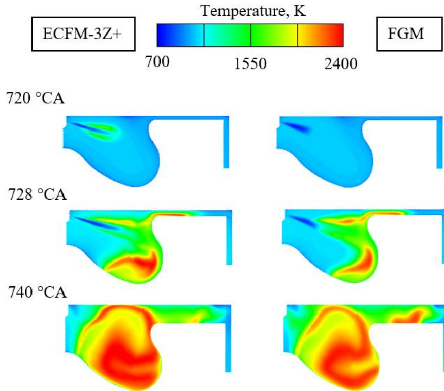
Figure 22. Temperature field for ECFM-3Z+ and FGM of the single-injection case
