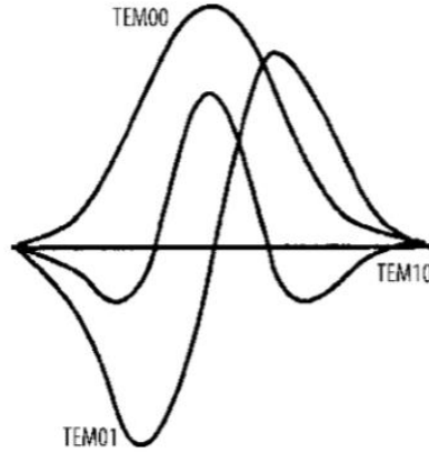
Figure 4 Amplitude variation for various modes [1]
