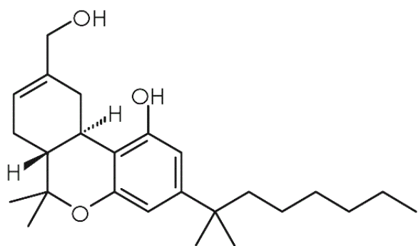
HU-210
