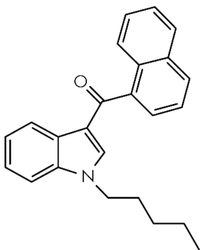
JWH-018
