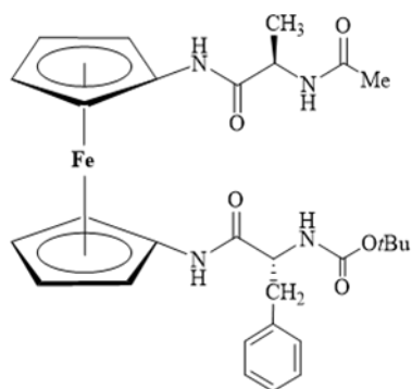
Ac-D-Ala-NH-Fn-NH-D-Phe-Boc (6)
