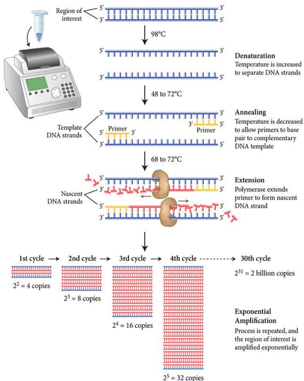
Figure 20. Quantitative real time polymerase chain reaction [from neb.com website]
