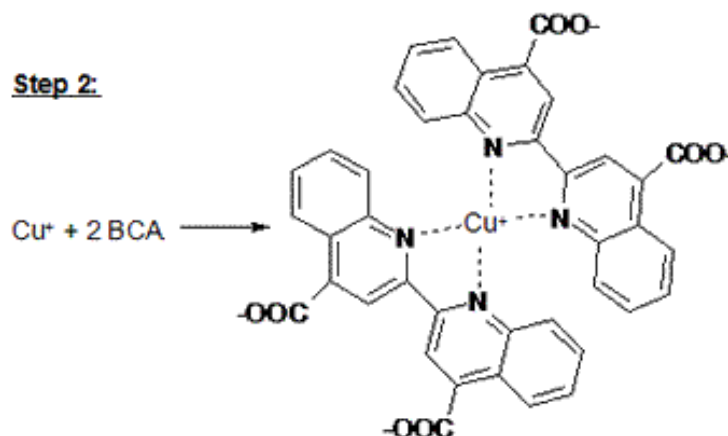
Figure 15. Reduction of \text{Cu}^{2+} and reaction with BCA forming purple-blue complex [from nfsc4500101groupa.weebly.com website]
