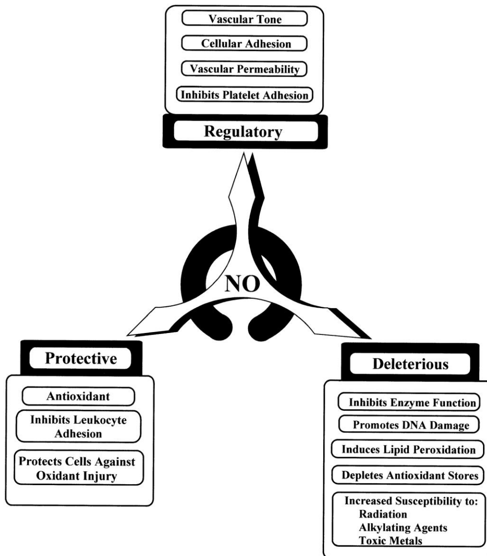
Figure 2. Roles of \text{NO}\cdot in mammals [from Grisham M. B. et al. 1999]
