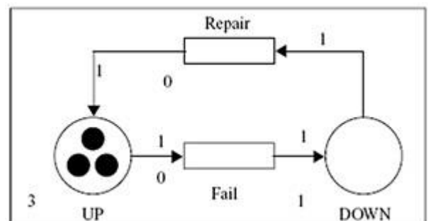
Figure 5. Stochastic Petri Net.
