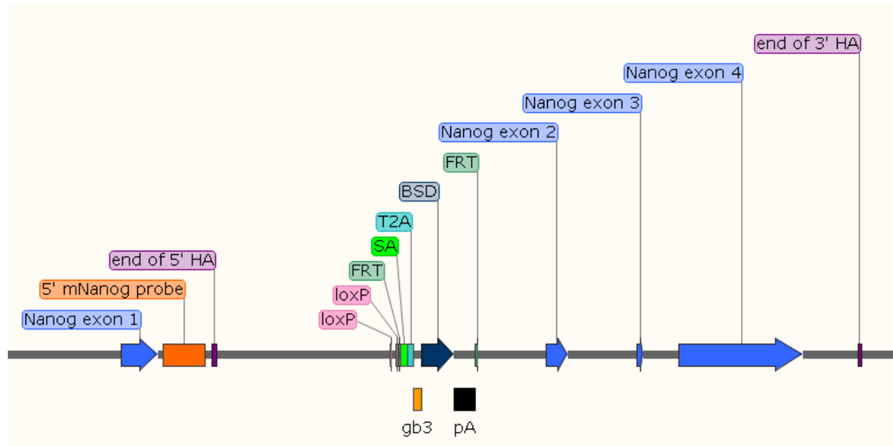
Figure 12. mNanog-Bsd-70 cassette inserted into the mNanog gene.
