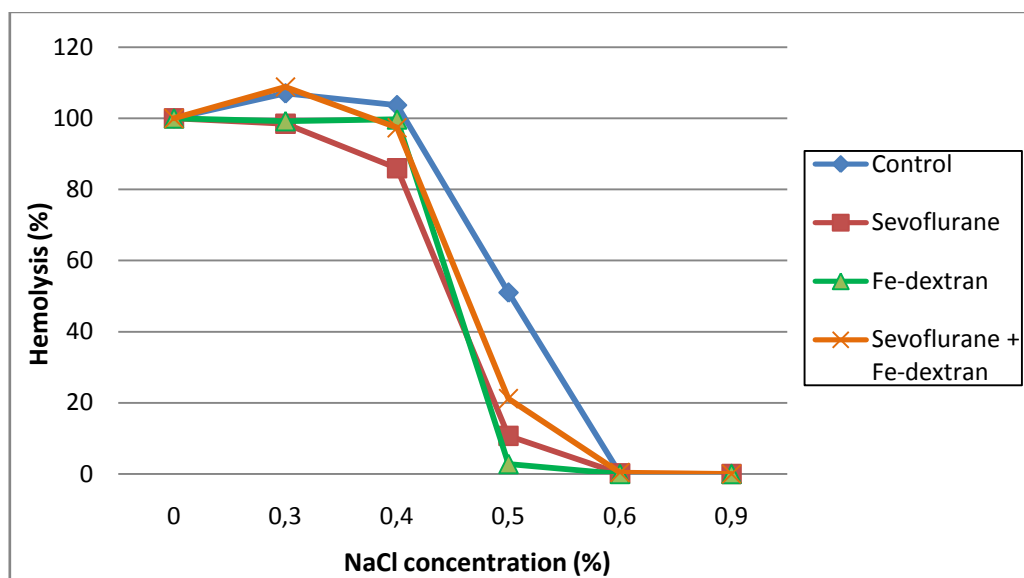
Figure 11. Changes in percentage of hemolysis in erythrocytes in Y59 rats treated with sevoflurane, iron-dextran and their combination. Rats ( n = 6 per group) were treated with 1.5 % Sevoflurane inhalation, injected ip with 50 mg/kg Fe-dextran and with combination of 1.5 % Sevoflurane and 50 mg/kg Fe-dextran (Sevoflurane inhalation was administered 2 h after Fe-dextran ip injection). Control group had saline solution (0.9 % NaCl) injected intraperitoneally. Animals were treated every other day for 21 days. Results are expressed as Mean + SE (SD).
