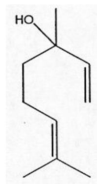
linalol
