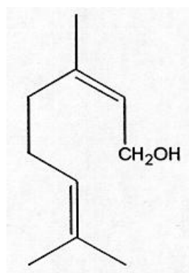
nerol
