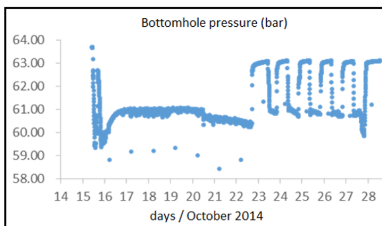
Figure 7-8 Variation of bottomhole pressure during the back-production test (WIESE B., 2014).
